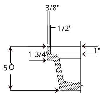
Water Dam Detail
