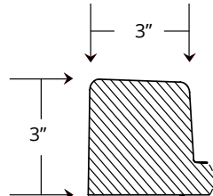
New, Solid Front Curb Detail
