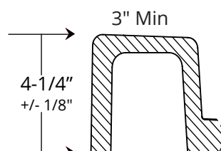
Front Curb Detail
