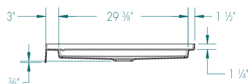
END VIEW
