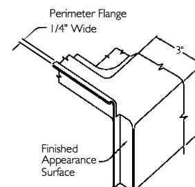
ISOMETRIC VIEW OF FRONT CORNER
