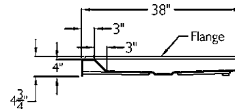
TOP VIEW OF FRONT CORNER
