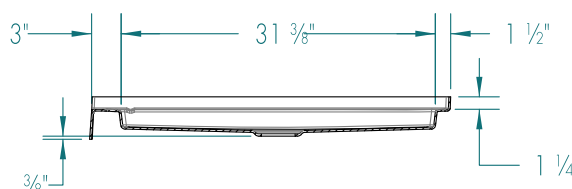
END VIEW
