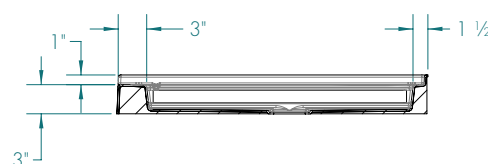
END VIEW
