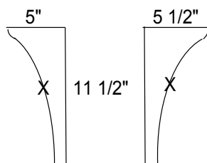
BRACKETS 1/2" THICK
