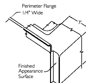
ISOMETRIC VIEW OF FRONT CORNER
