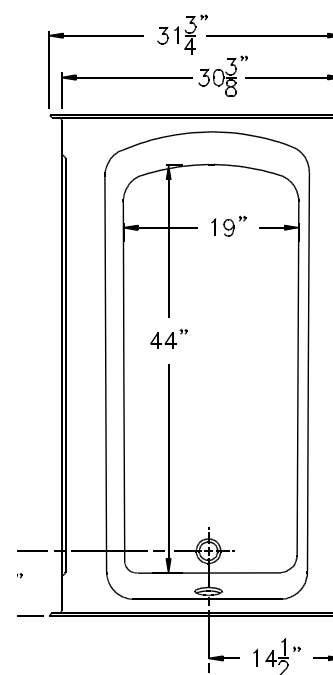
TOP VIEW
