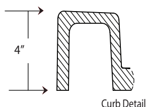
Curb Detail
