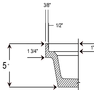
Water Dam Detail
