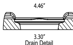
Drain Detail
