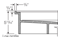
Flange Details: (U.S.)
