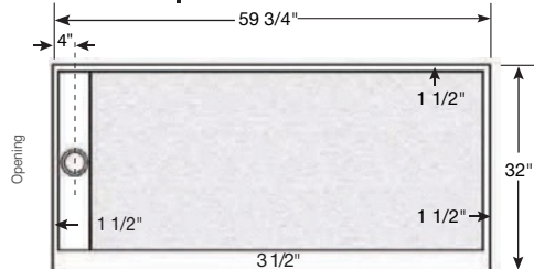
Top View - Left Drain
