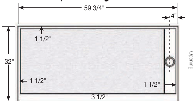
Top View - Right Drain
