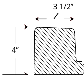
Front Treshold Detail
